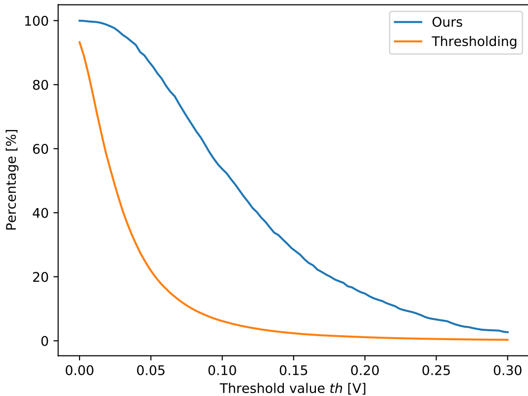
IoU vs threshold value th (worst case)
