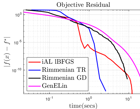
Figure 5: Generalized eigenvalue problem
