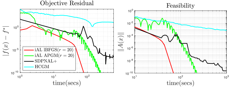
Figure 2: Convergence of different algorithms for k-Means clustering with fashion MNIST dataset. The solution rank for the template (32) is known and it is equal to number of clusters k (Theorem 1. [38]). As discussed in [62], setting rank r > k leads more accurate reconstruction in expense of speed. Therefore, we set the rank to 20.
