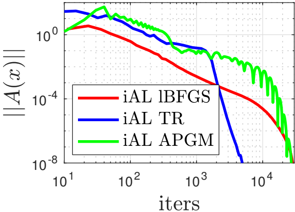
Feasibility Gap
