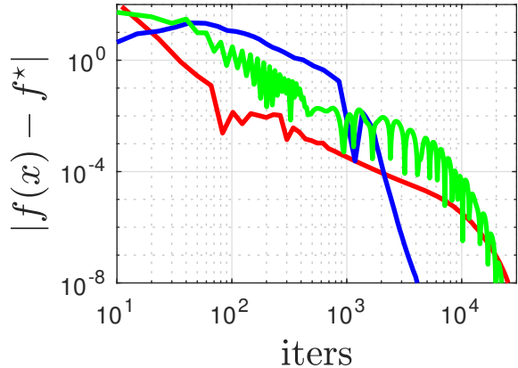
Objective Residual
