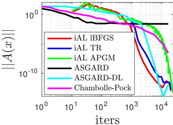
Feasibility Gap
