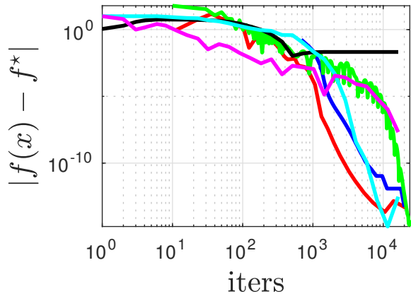
Objective Residual
