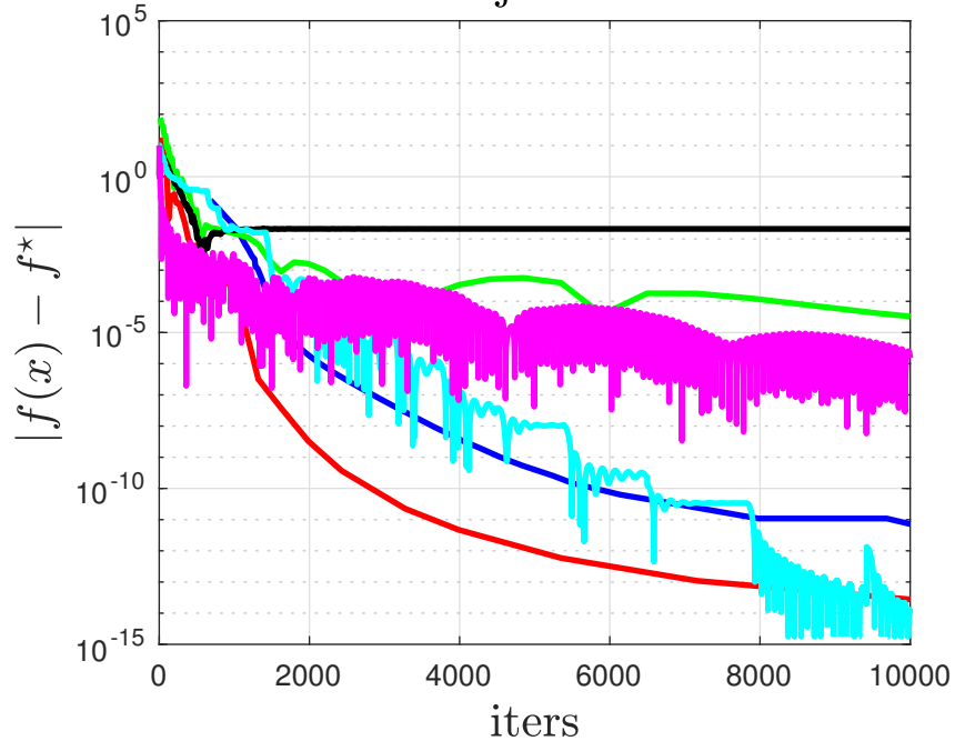
Relative Objective Residual
