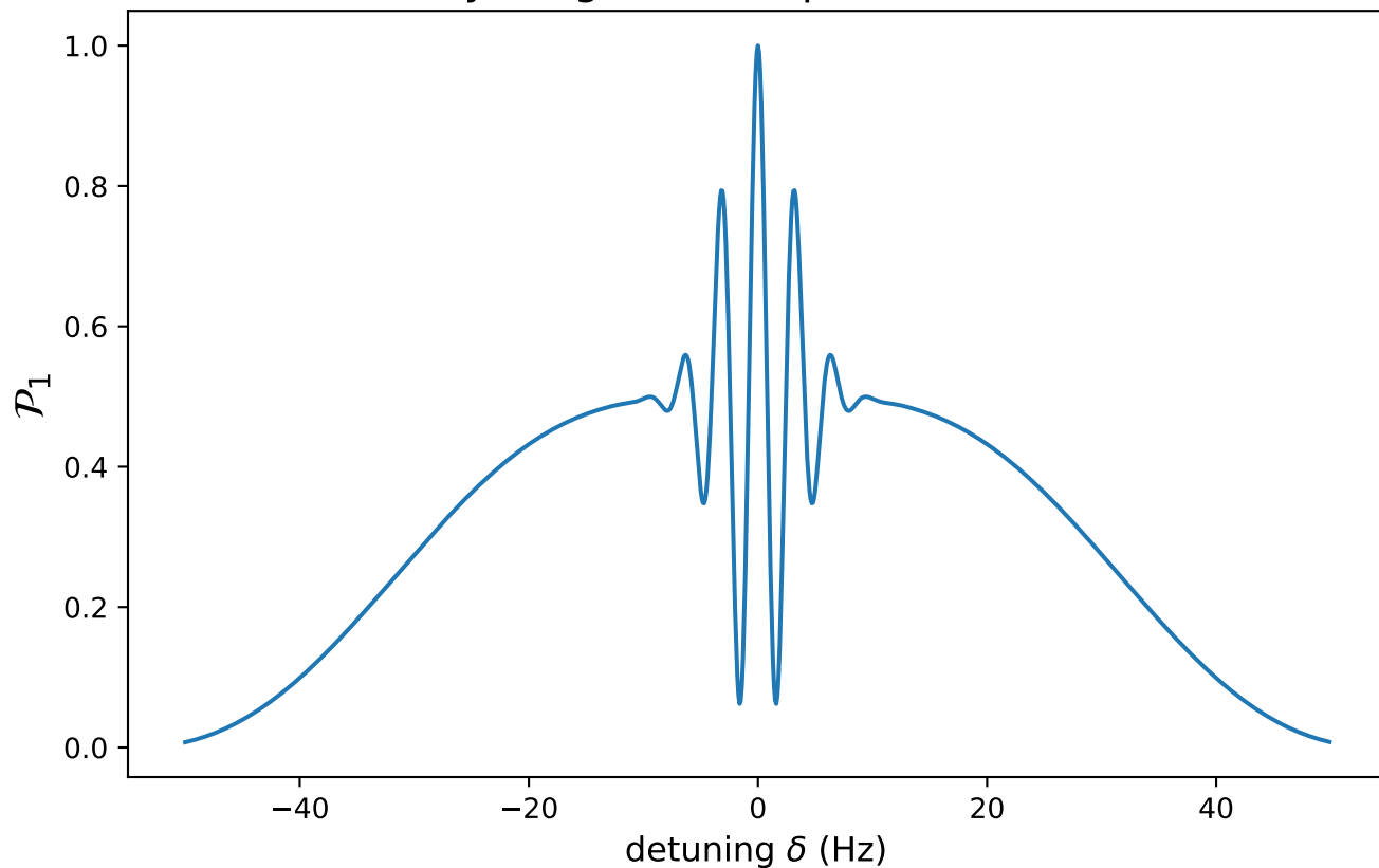
Ramsey fringes at temperature T = 1 mK
