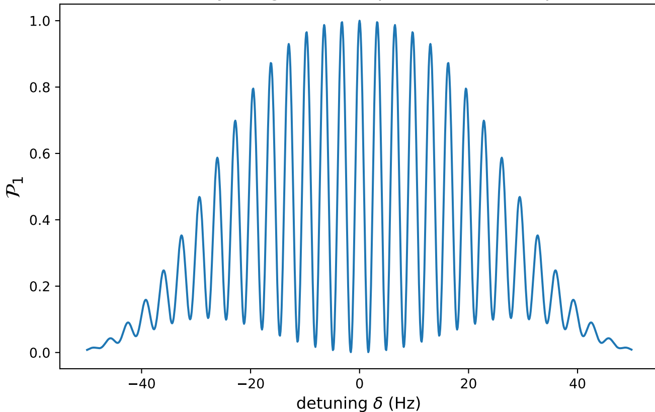
Ramsey fringes at temperature T = 10 \mu\text{K}
